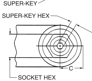
SOCKET END DETAIL
